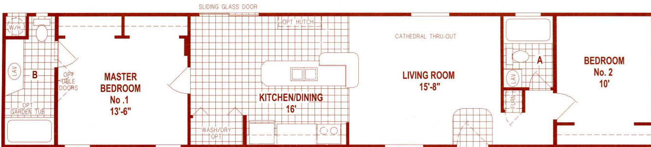
K305CT/6614 (902 SQ. FT.) 2BEDROOM - 2BATHS - CATHEDRAL THRU-OUT
