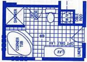
OPTION CORNER TUB BATH
