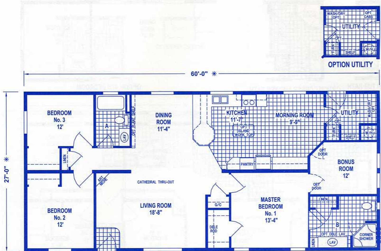
1246CT/6028 (1,620 SQ. FT.) 3BEDROOM - 2BATHS - CATHEDRAL THRU-OUT
